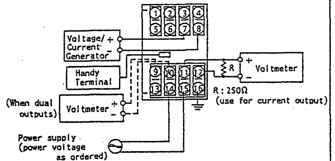
Fig.11 Connection to Handy Terminal
