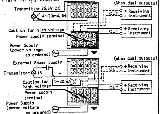
Fig.10 Wiring of Calibration Equipment
