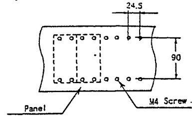
Fig.8 Terminal Arrangement
