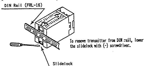
Fig.4 Mounting Block installation and removal
